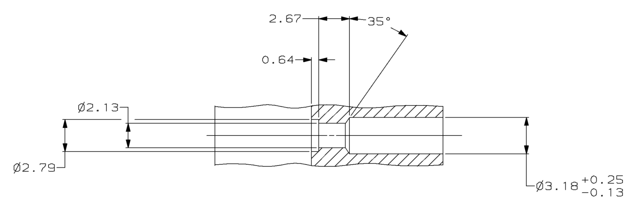
TYPICAL PLUG CAVITY SECTION (DIMENSIONS REFERENCE ONLY)
