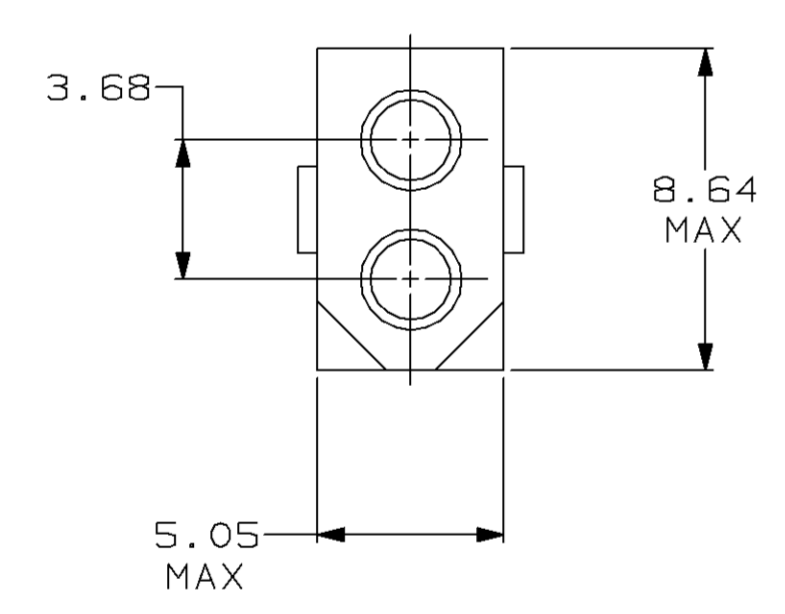
MATING CONNECTOR INTERFACE
